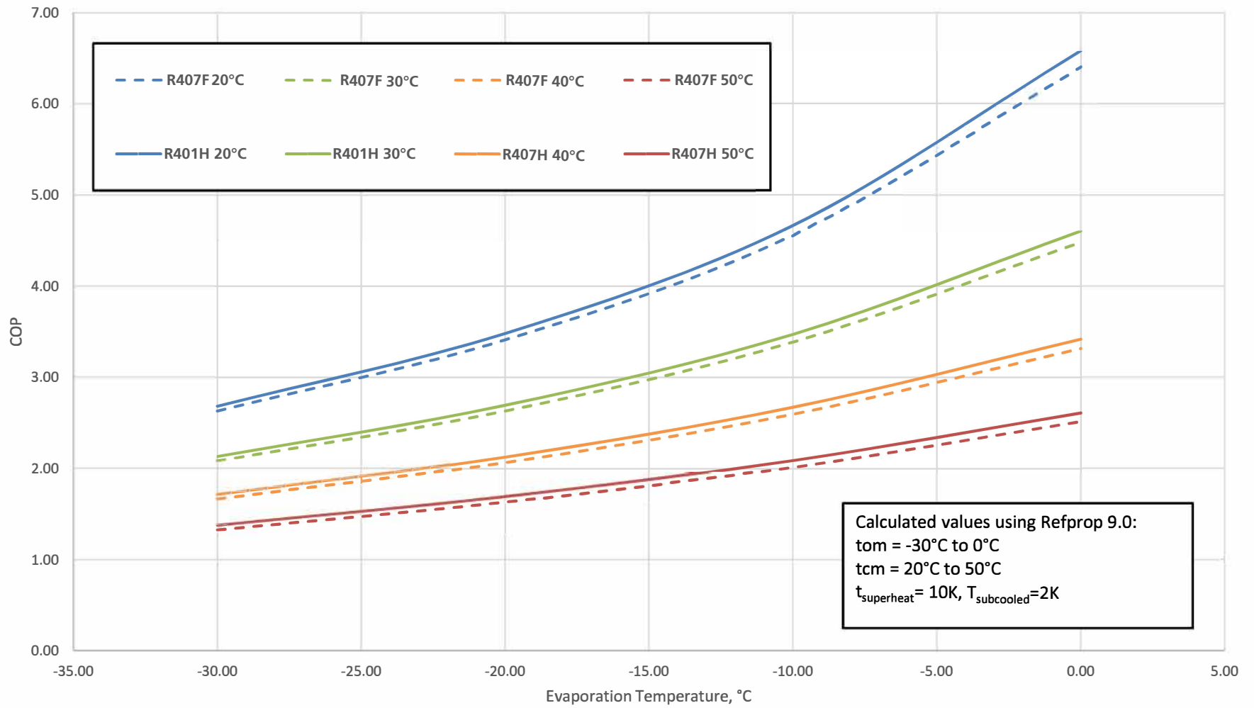
COP of R407F vs. R407H
